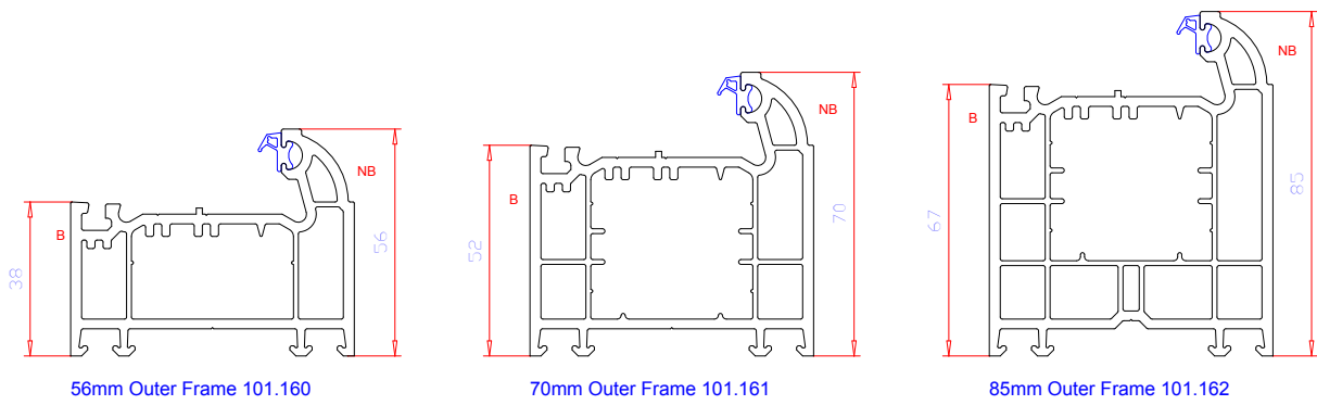
56mm Outer Frame 101.160
